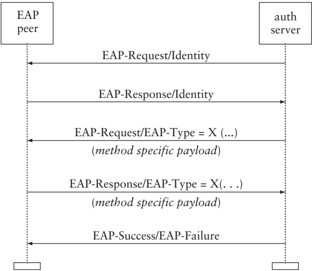
○ Figure 16.13: EAP Generic Message Flow
